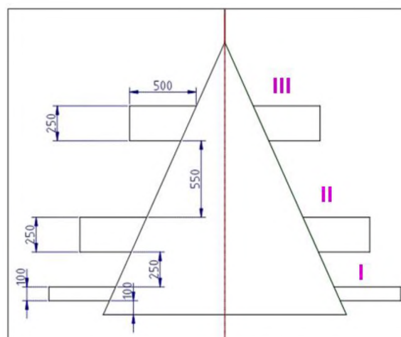
Schematic diagram of vertical troughs of IVNFS (all dimensions are in mm)
