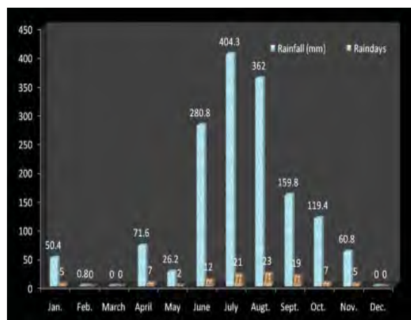
Fig. 71. Rainfall distribution
